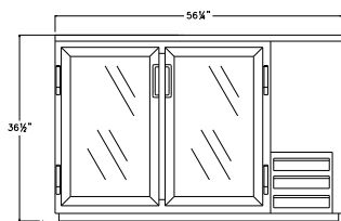
Vista Frontal / Front View
